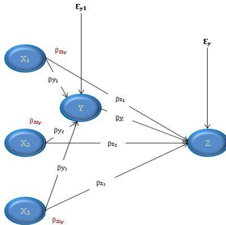
Figure 3. Research Constellation
