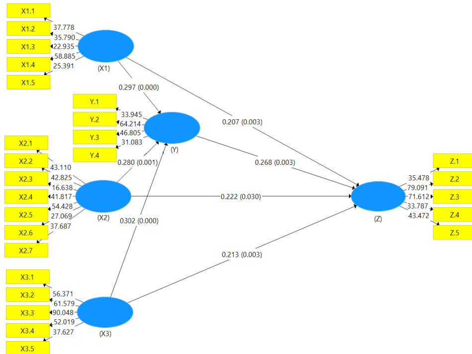
Figure 4. Research Constellation
